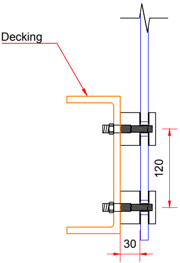
CONNECTION TO STEEL BEAM
