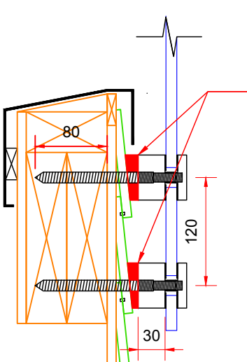
CONNECTION TO WEATHER BOARD
