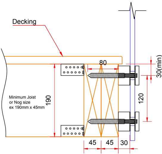
CONNECTION TO TIMBER
