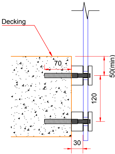
CONNECTION TO CONCRETE
